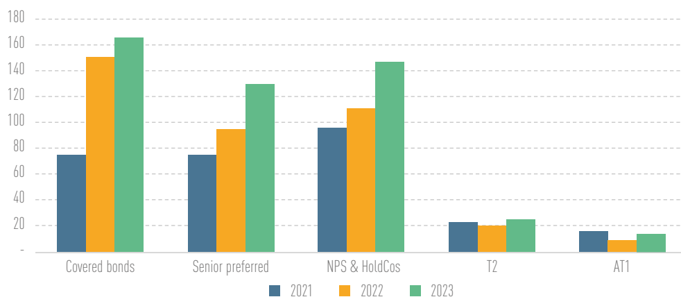
Figure 41: Issuance volumes of EU/EEA banks’ debt and capital instruments, Q1 – Q3 2021 – 2023 (in EUR bn) [51]
